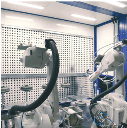
➤ Continuous automatic liquid painting systems with floor conveyor
